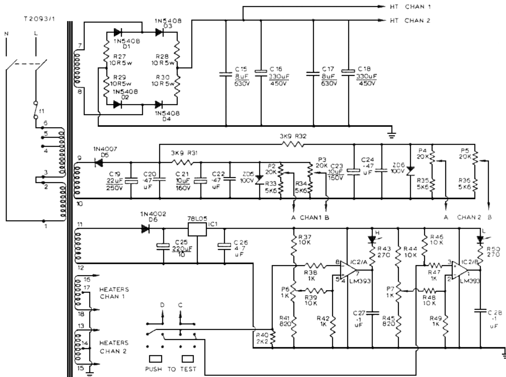
Fig.3 Power Supply Circuit STA25 Renaissance
